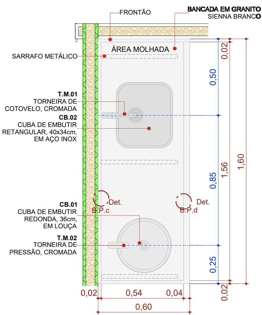
BPC.160d Escala:1:20
