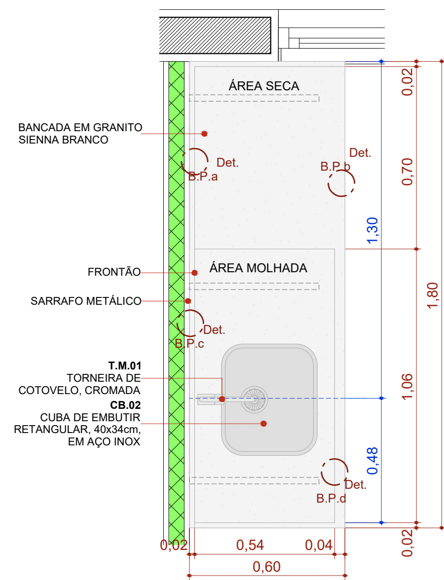
BPC.180d Escala:1:20
